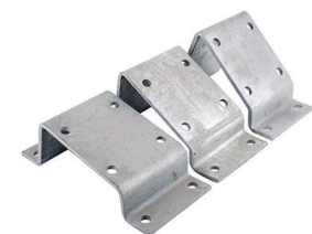
Wall attachments (articles no 23104, 23106, 23107)
